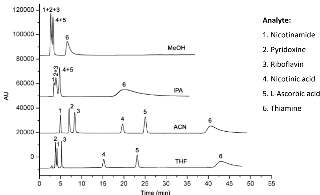
Fig. 2. Effect of organic modifier on separation of the WSV. Conditions: Inertsil diol column with 10:90 (v/v) aqueous ammonium acetate buffer (10 mM, pH 5.0)—organic solvent as mobile phase; flow rate 0.6 mL min -1 ; column temperature 25 °C. 1 = nicotinamide, 2 = pyridoxine, 3 = riboflavin, 4 = nicotinic acid, 5 = L-ascorbic acid, 6 = thiamine
